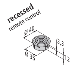
flush-mounted touch remote control
